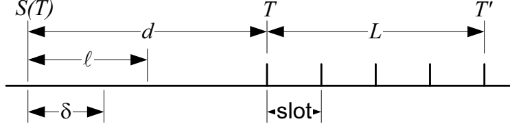
Fig. 1. Random variables used in the FCFS analysis
