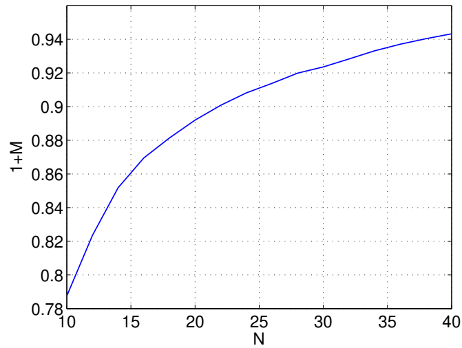
Fig. 2. 1 + M as a function of the number of observations N when estimating an SNR of 2.
