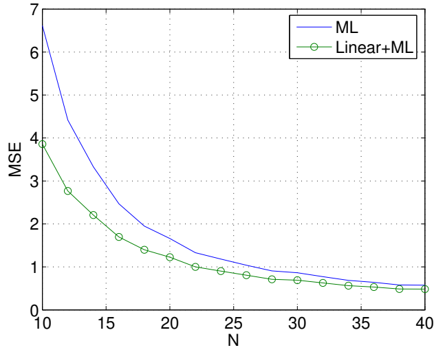
Fig. 1. MSE in estimating the SNR as a function of the number of observations N for an SNR of 2 using the ML and the linearly transformed ML estimators.
