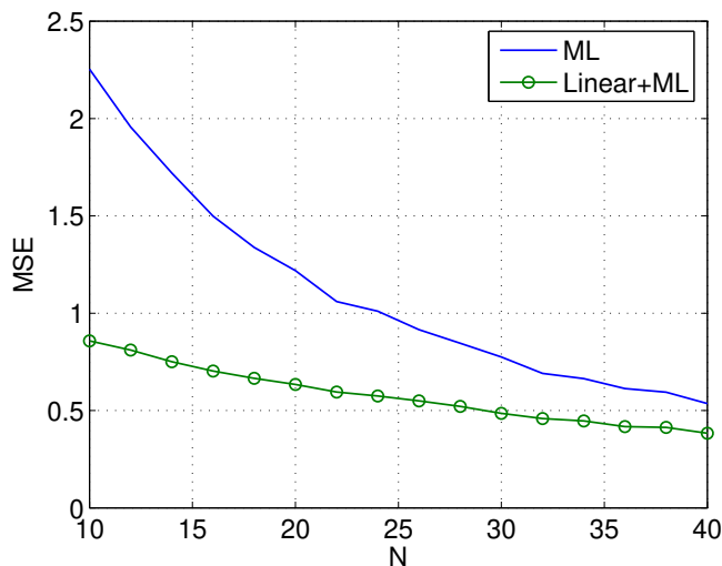
Fig. 3. MSE in estimating the SNR as a function of the number of observations N for an SNR of 2 using the ML and the linearly transformed ML estimators subject to the constraint (96).
