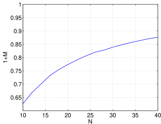
Fig. 4. 1 + M as a function of the number of observations N when estimating an SNR of 2 subject to the constraint (96).
