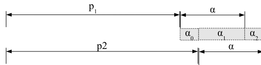
Figure 1: Breakdown of \alpha in Lemma 3.
