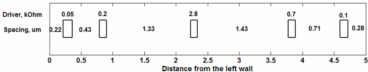
Fig. 9 A bundle with uniform timing requirements; a) Cross section after weighted sum minimization without ordering; b) Cross section after weighted sum of delays minimization with ordering (symmetric hill order according to driver resistances)
