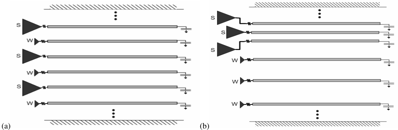
Fig. 2 Space sharing in two interconnects channel configurations. a) Interleaved placement of strong and weak drivers, b) Sorted placement of signals according to driver strength.
