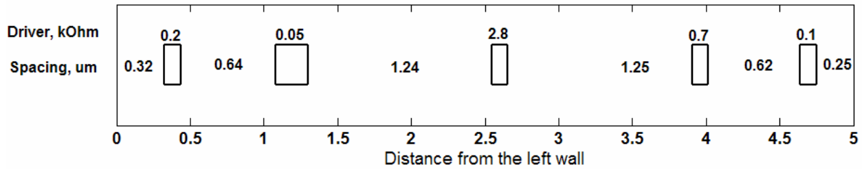
Fig. 10 A bundle with a critical wire; a) Cross section after weighted sum minimization without ordering (the critical wire is at the leftmost position); b) Cross section after weighted sum minimization with ordering (symmetric hill order according to effective signal resistance)
