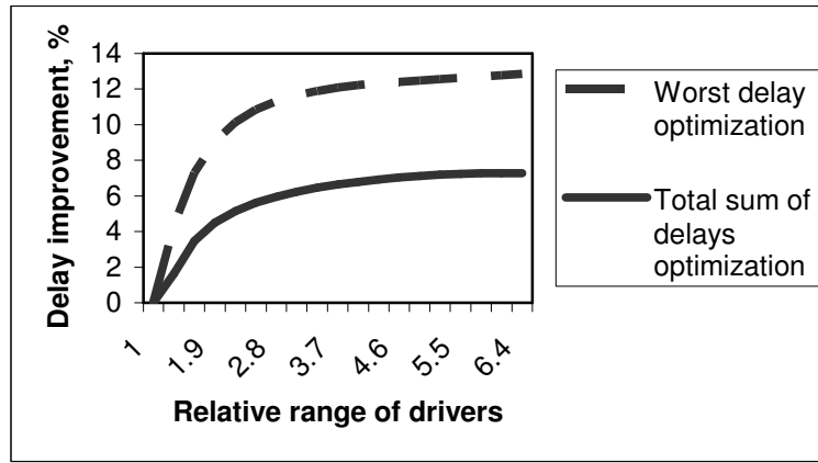
Fig. 8. Influence of relative range of drivers on optimization impact
