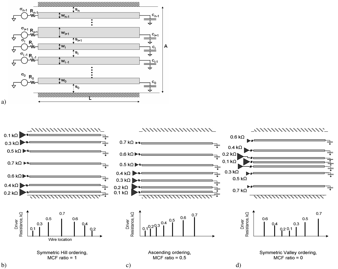
Fig. 1. (a) Signal drivers (modeled as voltage sources with series resistances), interconnect bundle wires of length L , and receivers (modeled as load capacitances). Timing optimization is performed by reordering the signal wires and by allocating wire widths and spaces, for a given constrained channel width A . (b, c, d) present the optimal order of signals and the corresponding wire-to-wire space allocation for various ratios of MCF between extreme and internal signals.
