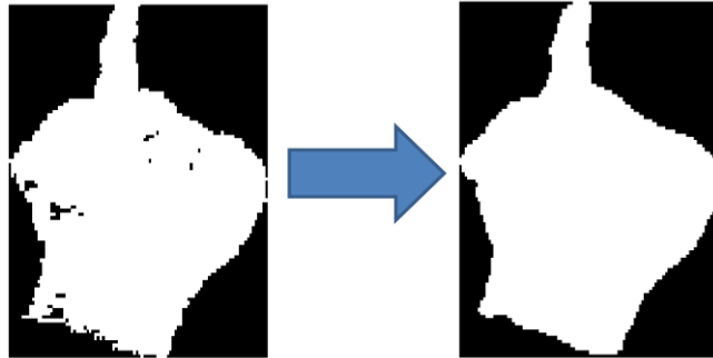
Figure 6 - Median filter
