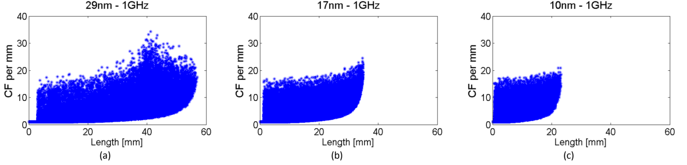
Figure 4. Results of Monte-Carlo analysis of interconnect cost, subject to CF (7) with \alpha=\beta=0.5 , for 29nm, 17nm and, 10nm technology nodes (a,b,c respectively) and a target clock frequency of 1GHz.
