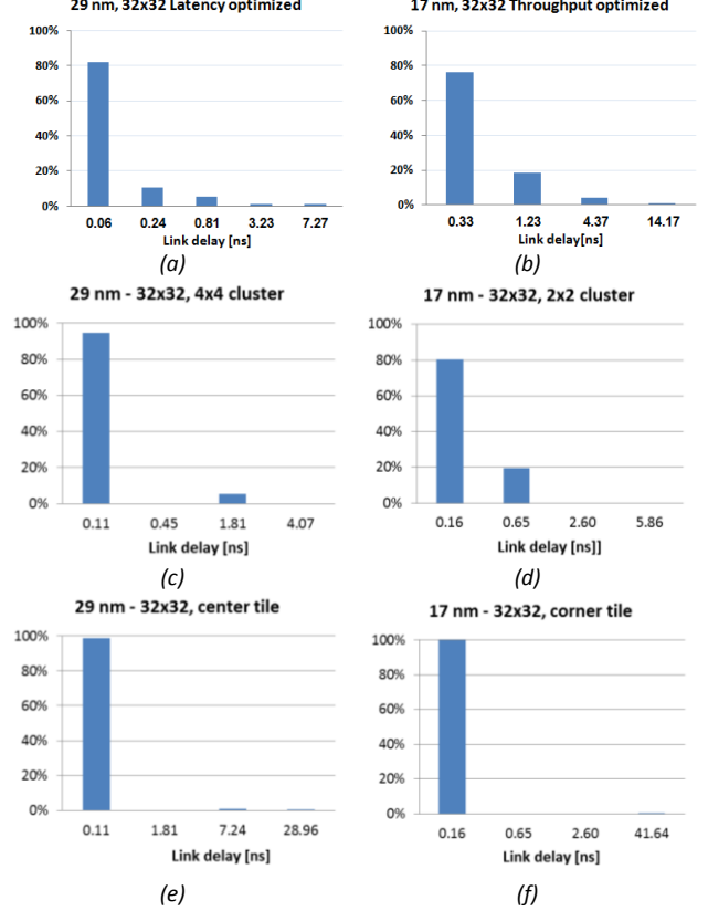
Figure 9. Six examples of minimum size global links delay histograms: (a) – 32x32 delay optimized PyraMesh at 29nm. (b) – 32x32 throughput optimized PyraMesh at 17nm. (c) – 32x32 hierarchical NoC with 4x4 clusters at 29nm. (d) – 32x32 hierarchical NoC with 2x2 clusters at 17nm. (e) – 32x32 Ring of meshes with a center located ring interconnect. (f) – 32x32 Ring of mesh with a corner located ring interconnect. Each bin indicates the ratio in % out of all NoC links.
