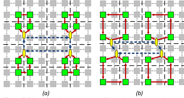
Figure 7. Ring of meshes. (a) – corner tile used to connect to the ring. (b) – center tile used. Red and blue arrows represent the lower and the upper ring respectively. The green squares represent mesh-lower ring connections and the yellow ellipses – the connection between lower and upper level rings.
