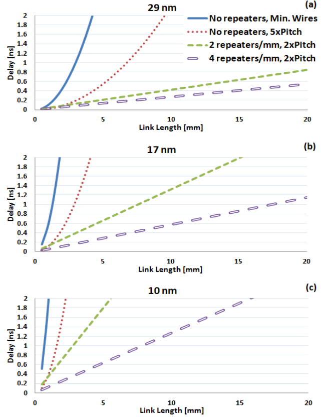
Figure 3. The four configurations presented are: I-Minimal size wires without repeaters, II-Wires with \Lambda_W=\Lambda_S=5 and no repeaters, III- \Lambda_W=\Lambda_S=2 with 2 repeaters/mm, IV- Wires with \Lambda_W=\Lambda_S=2 with 4 repeaters/mm. (a)-(c) present 29, 17 and 10 nm technology nodes respectively.
