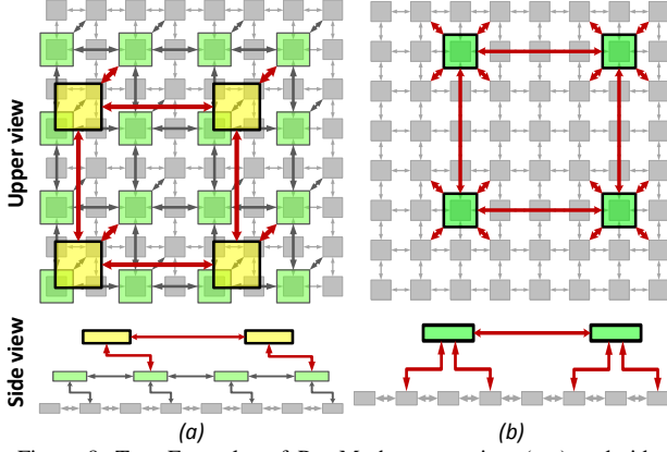
Figure 8. Two Examples of PyraMesh, upper view (top) and side view (bottom). (a) – 3-levels PyraMesh with (K = 8, NP = 1, NL = 3, \alpha = 2 , C = 1). (b) – 2-levels PyraMesh with (K = 8, NP = 1, NL = 2, \alpha = 4 , C = 2). The upper view figures are taken from [1].
