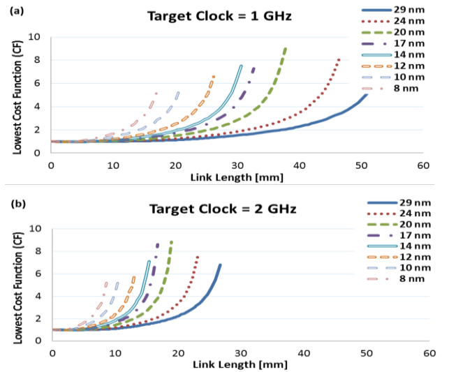
Figure 5. Minimal cost function for different technologies, (a)-for 1GHz and (b)-2GHz operating frequencies.
