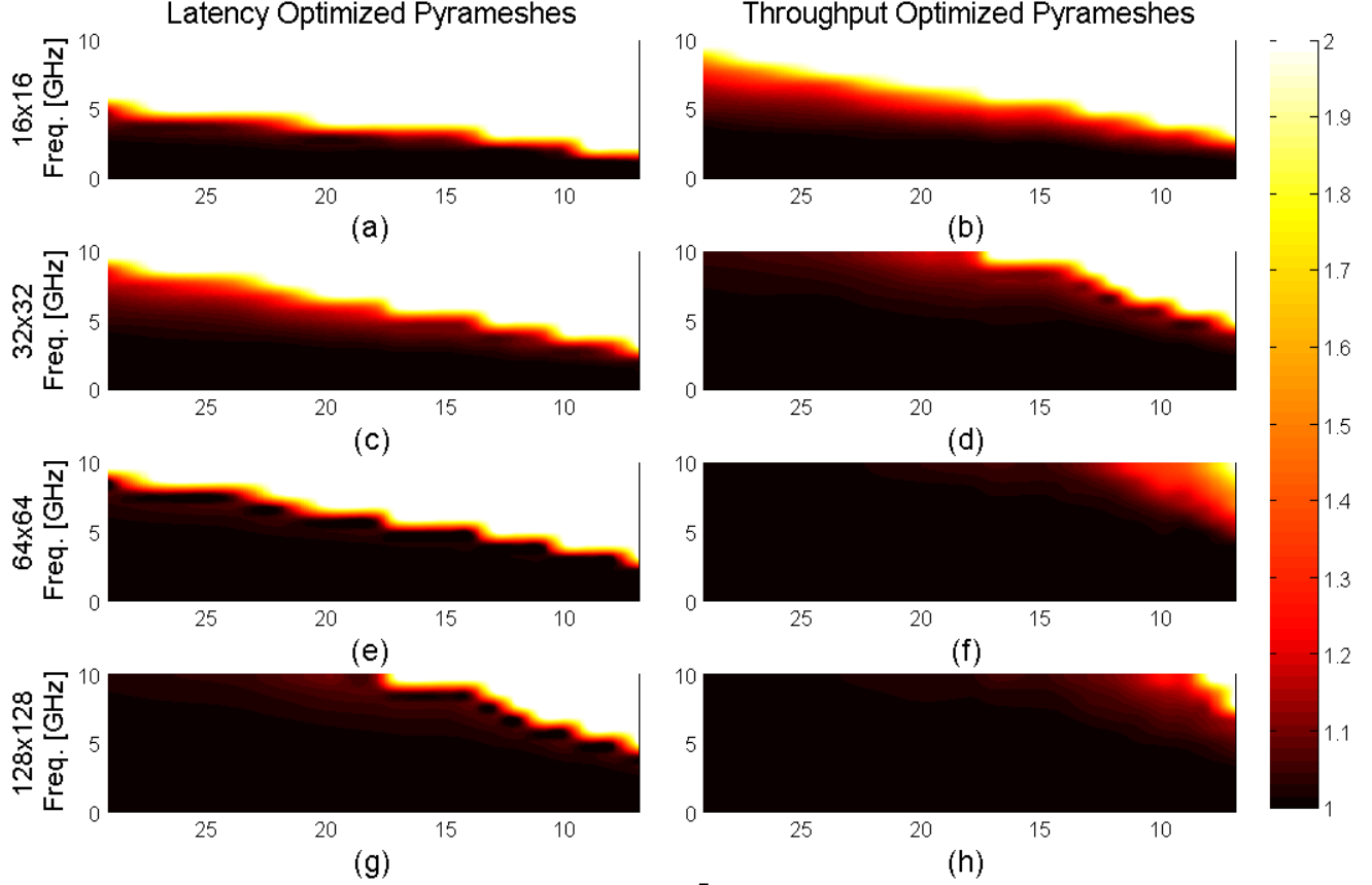
Figure 10. NIO for different target clocks at different technologies. Latency optimized and throughput optimized PyraMeshes are presented in figures (a,c,e,g) and (b,d,f,h) respectively; Baseline mesh sizes: 16x16 (figures a and b), 32x32 (c, d), 64x64 (e, f) and 128x128 (g, h).
