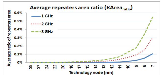
Figure 11. Average RArea_{ratio} for 1, 2 and 3 GHz target clocks, for various technology nodes.
