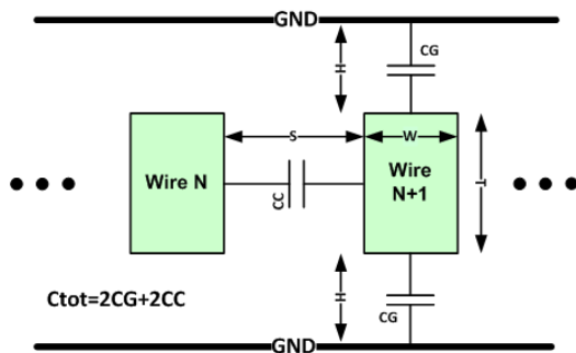
Figure 2. Interconnect physical model.
