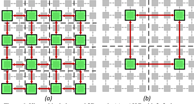
Figure 6. Hierarchical clustered 2D mesh. (a) – AHC with 2x2 clusters. (b) – Real clusters with 4x4 cluster size.
