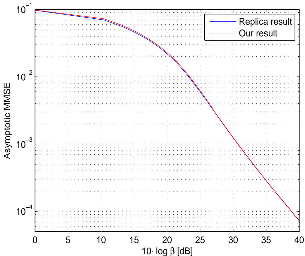
Fig. 2. Comparison of the asymptotic MMSE using Theorem 1 and the replica method as a function of \beta , for sparsity rate p = 0.1 , and measurement rate R = 0.3 .
